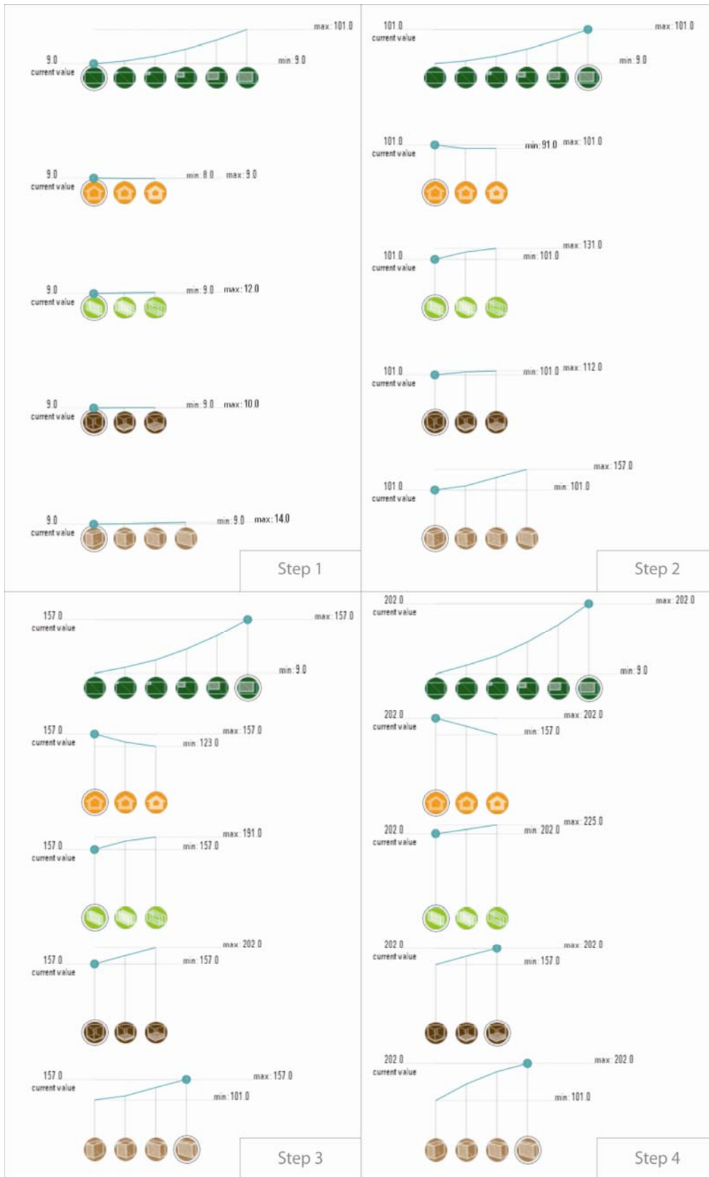
Figure 5 – A typical example of an optimization sequence for Useful Solar Gains(USG). This maximization involves navigating through parameter space first along the Glazing Ratio, Aspect Ratio, and finally Thermal Mass dimensions.
