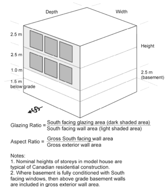
Figure 2 – Example of base house model for generating parametric performance simulations.
