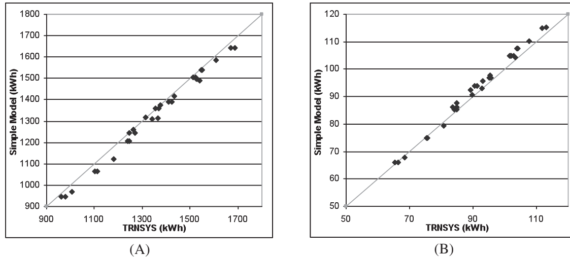
FIGURE 1: VALIDATION OF SIMPLE MODEL SHOWING (A) PREDICTED ANNUAL INCIDENT SOLAR RADIATION ON THE PV PANEL AND (B) PREDICTED ANNUAL ELECTRICITY GENERATION
