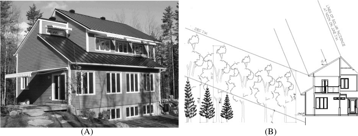
FIGURE 3: (A) A PHOTOGRAPH OF THE ECOTERRA HOUSE, FEATURING A BUILDING-INTEGRATED PV/THERMAL (BIPV/T) SOLAR COLLECTOR COVERING THE ENTIRE UPPER ROOF. 21 LONG FLEXIBLE AMORPHOUS SILICON PANELS ARE FIXED TO THE METAL ROOF. (B) ARCHITECTURAL DRAWINGS OF SOLAR ALTITUDE ON DECEMBER 21 AND JUNE 21 AT SOLAR NOON.
