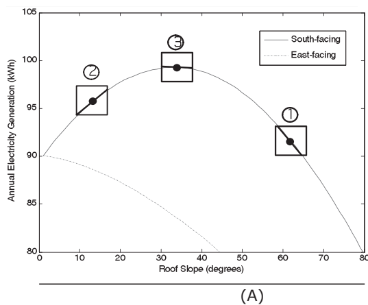
FIGURE 4: (A) EXAMPLE OF LINES OF INFLUENCE. (B) EXAMPLE OF REDUCING DESIGN SPACE TO FEASIBLE DESIGNS AND IMPLICATIONS
