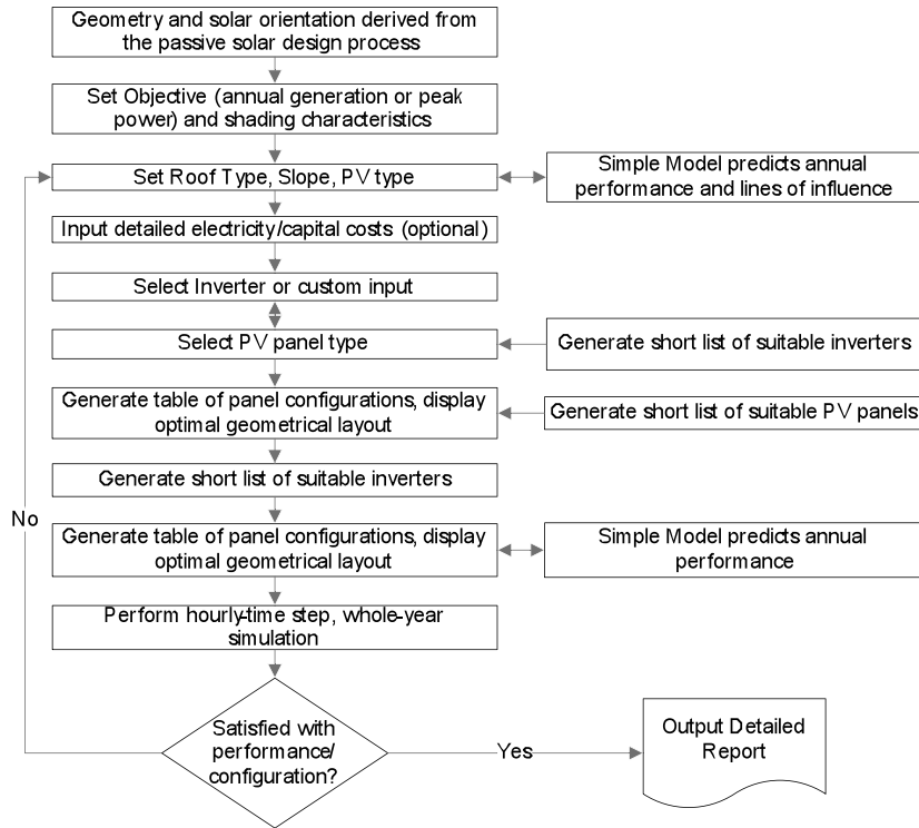
FIGURE 5: HIGH-LEVEL ROOF DESIGN PROCEDURE
